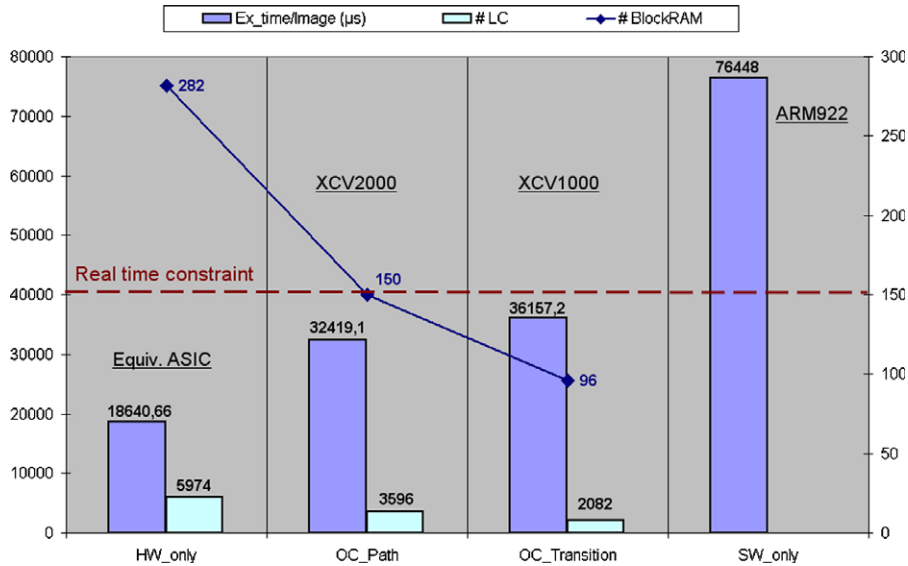
Fig. 14. Execution time/image and resource use.
