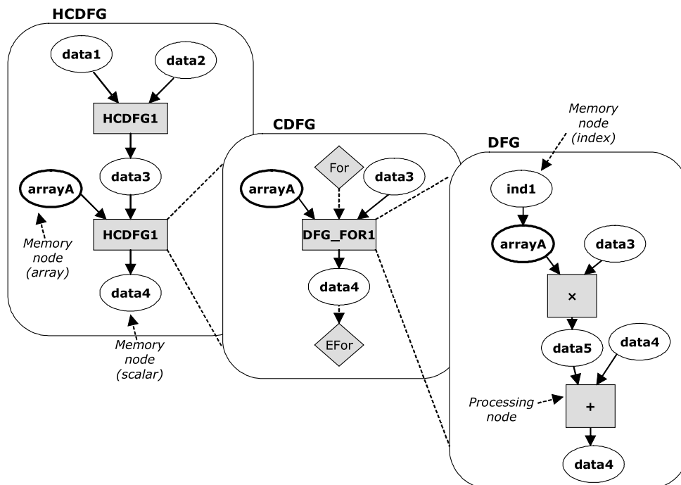
Fig. 5. A HCDFG specification example.
