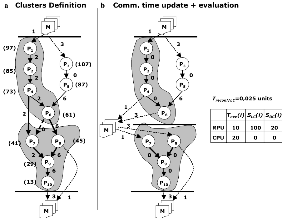
Fig. 11. Our clustering heuristic.
