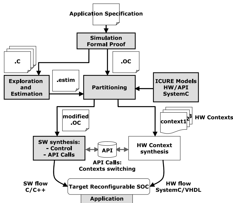
Fig. 3. EPICURE global design flow.
