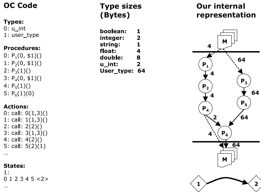
Fig. 8. Data dependency check and DFG construction.
