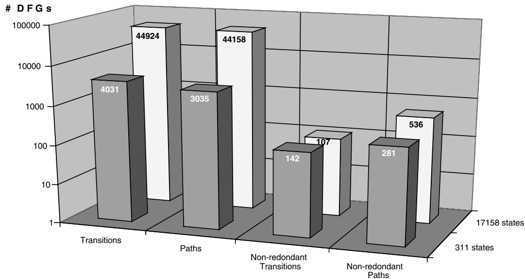
Fig. 17. DFG redundancy reduction.
