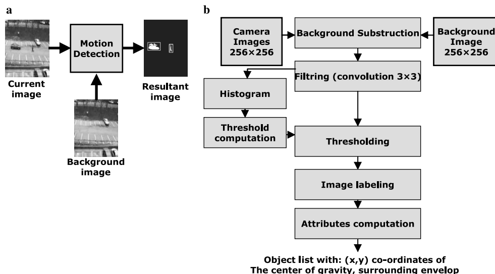
Fig. 12. The ICAM video supervision application.
