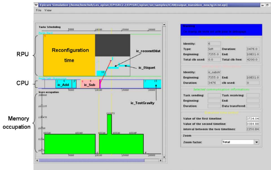
Fig. 13. A partitioning solution over a transition.
