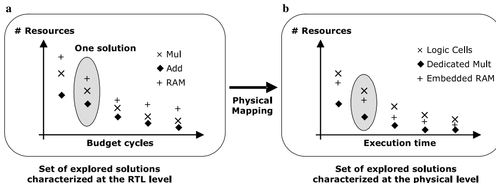
Fig. 6. HW tradeoff curves – parallelism exploration.
