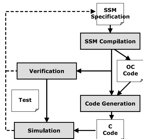
Fig. 2. Compilation flow using OC.
