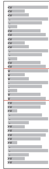
Overview of 3-way string quicksort
