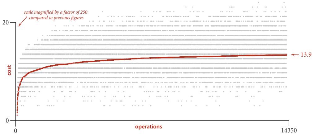
Costs for java FrequencyCounter 8 < tale.txt using BST
