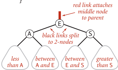
Flipping colors to split a 4-node
