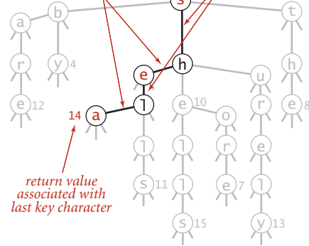
TST search example
