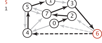
Trace of the Bellman-Ford algorithm (negative weights)
