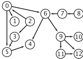
Standard digraph model
