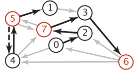
Trace of the Bellman-Ford algorithm (negative cycle)
