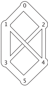
add 2 units of flow along 0->1->3->5
