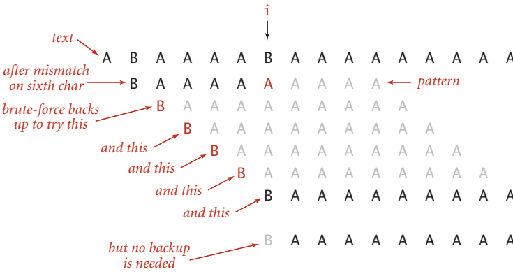
Text pointer backup in substring searching
