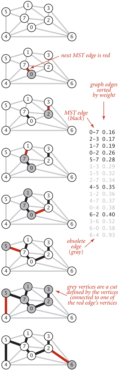
Trace of Kruskal's algorithm
