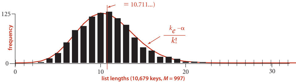
List lengths for java FrequencyCounter 8 < tale.txt using SeparateChainingHashST
