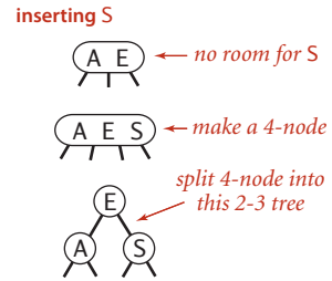
Insert into a single 3-node
