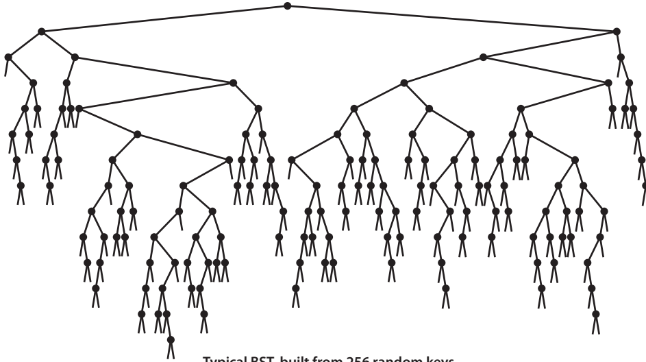
Typical BST, built from 256 random keys
