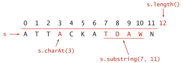
Fundamental constant-time String operations
