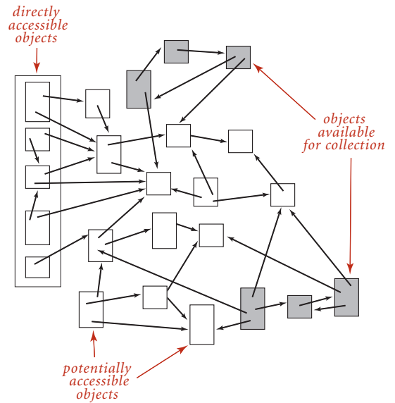
Garbage collection scenario
