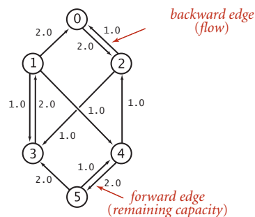
Anatomy of a network-flow problem (revisited)
