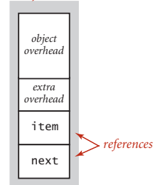
Typical object memory requirements
