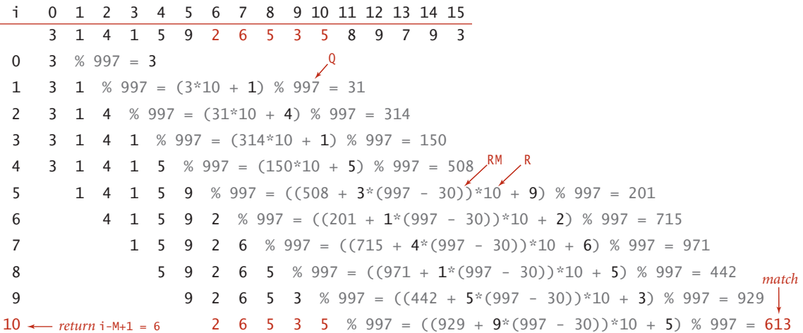
Rabin-Karp substring search example
