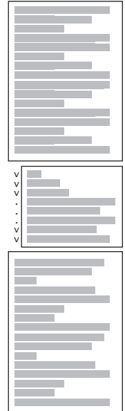
Overview of 3-way string quicksort
