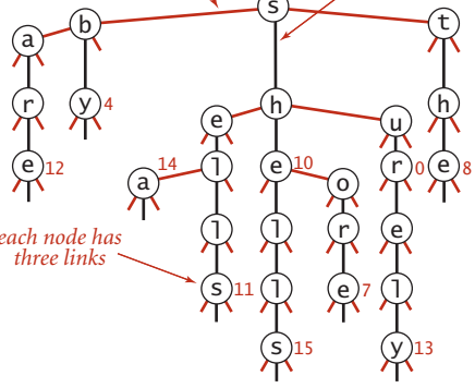
TST representation of a trie
