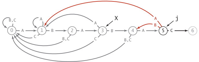
Constructing the DFA for KMP substring search for A B A B A B A C
