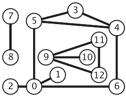
Two drawings of the same graph
