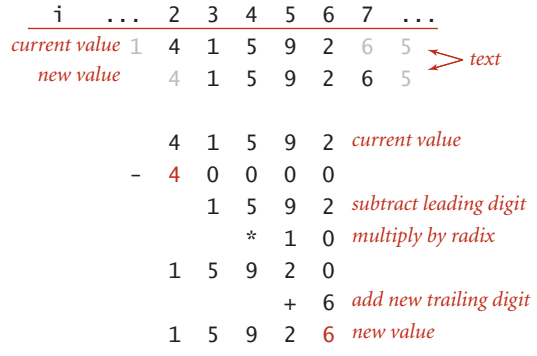
Key computation in Rabin-Karp substring search (move right one position in the text)
