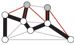
A cut with two MST edges
