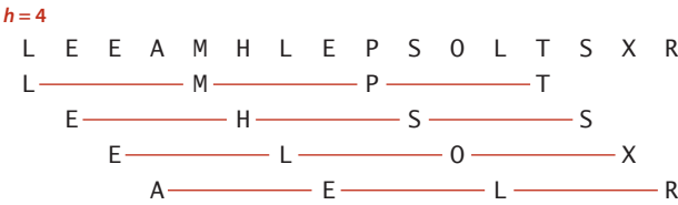
An h -sorted sequence is h interleaved sorted subsequences
