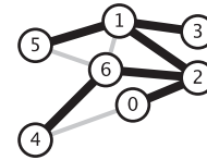
weights can be 0 or negative
