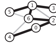
MST may not be unique when weights have equal values
