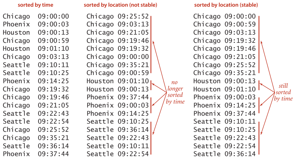
Stability when sorting on a second key
