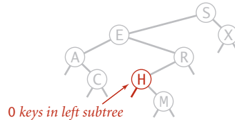
Selection in a BST
