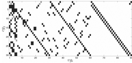
Fig. 7. New base DVb-T2 Matrix after factor 2 split
